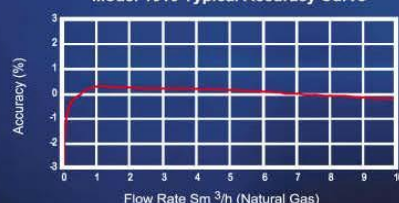
Model 1010 Typical Accuracy Curve
